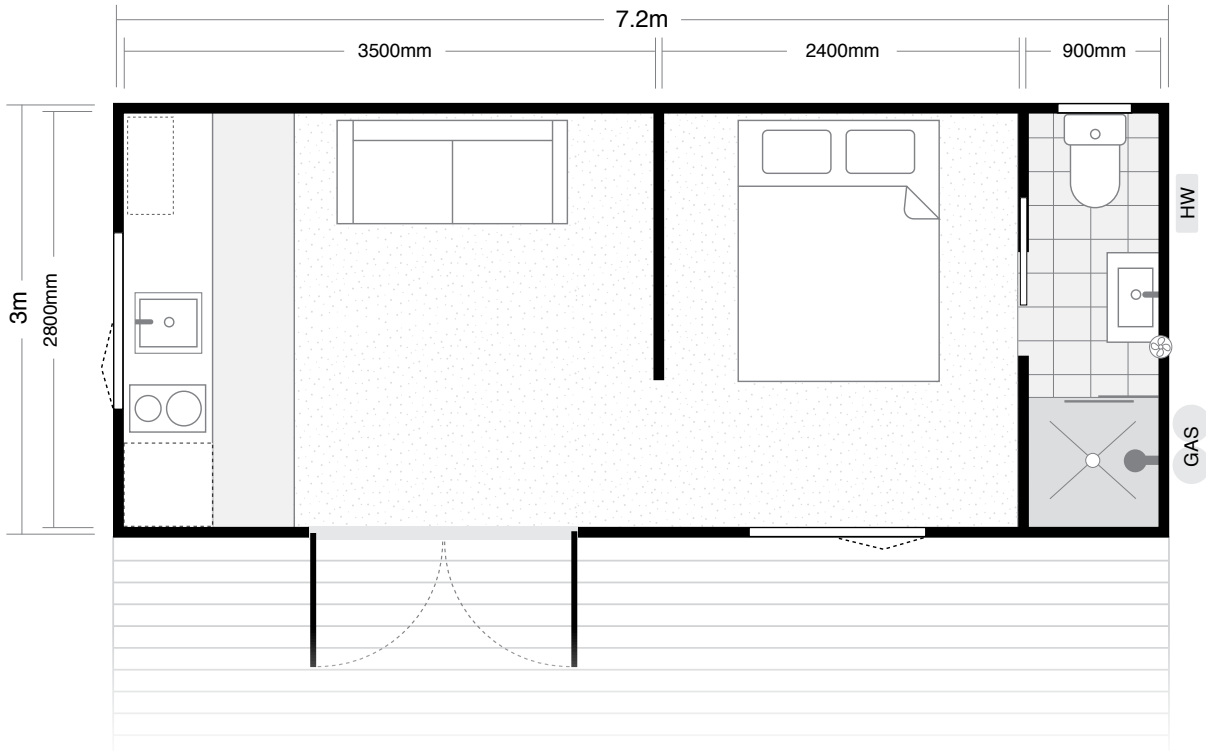
Floor plan drawing is not to scale. Decking shown is an added extra. Furniture shown is for demonstration purposes only.
